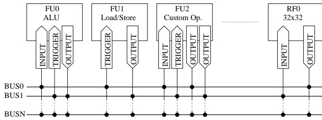
Fig. 1. Example of a TTA processor.
